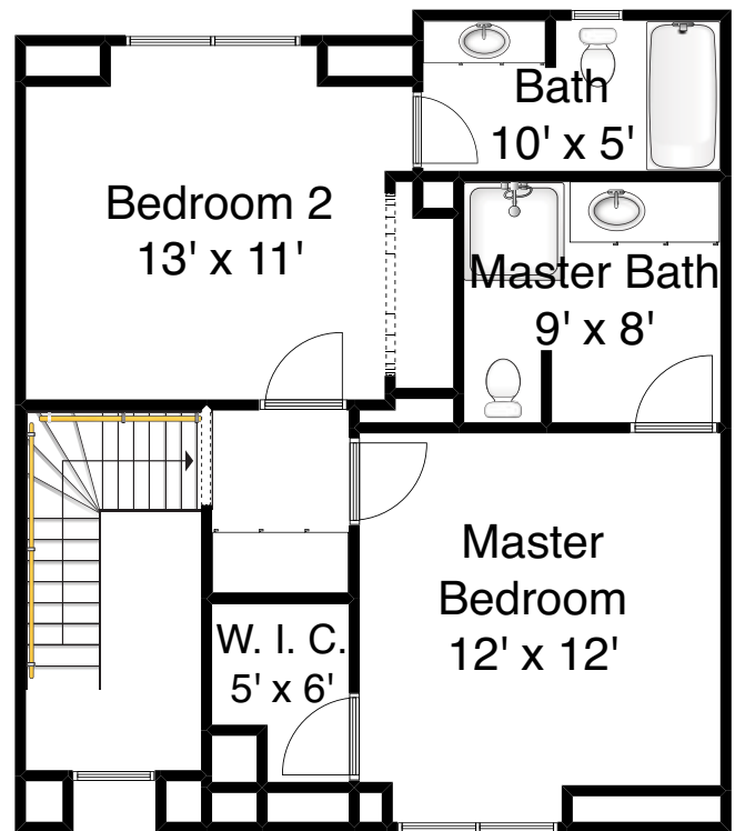
UPPER LEVEL
